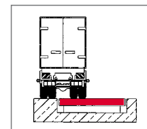
Top reinforcement for transit of truck
