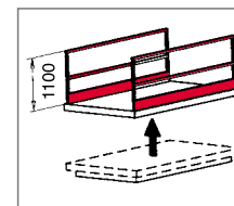
Safety handrails
