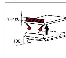
Roll-off stop
